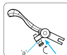
Screw Adjust
